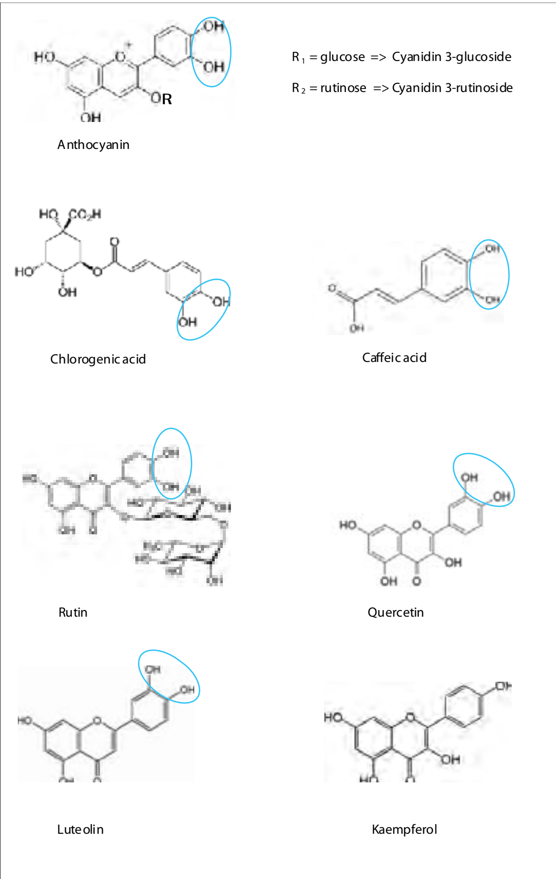
Figure 4. Molecular structures of phenolic compounds detected in Tasmania Pepper Berry indicated catechol structure is necessary for antioxidant properties of a phenolic compound [15]
