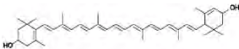
Figure 7. Molecular structure of lutein
